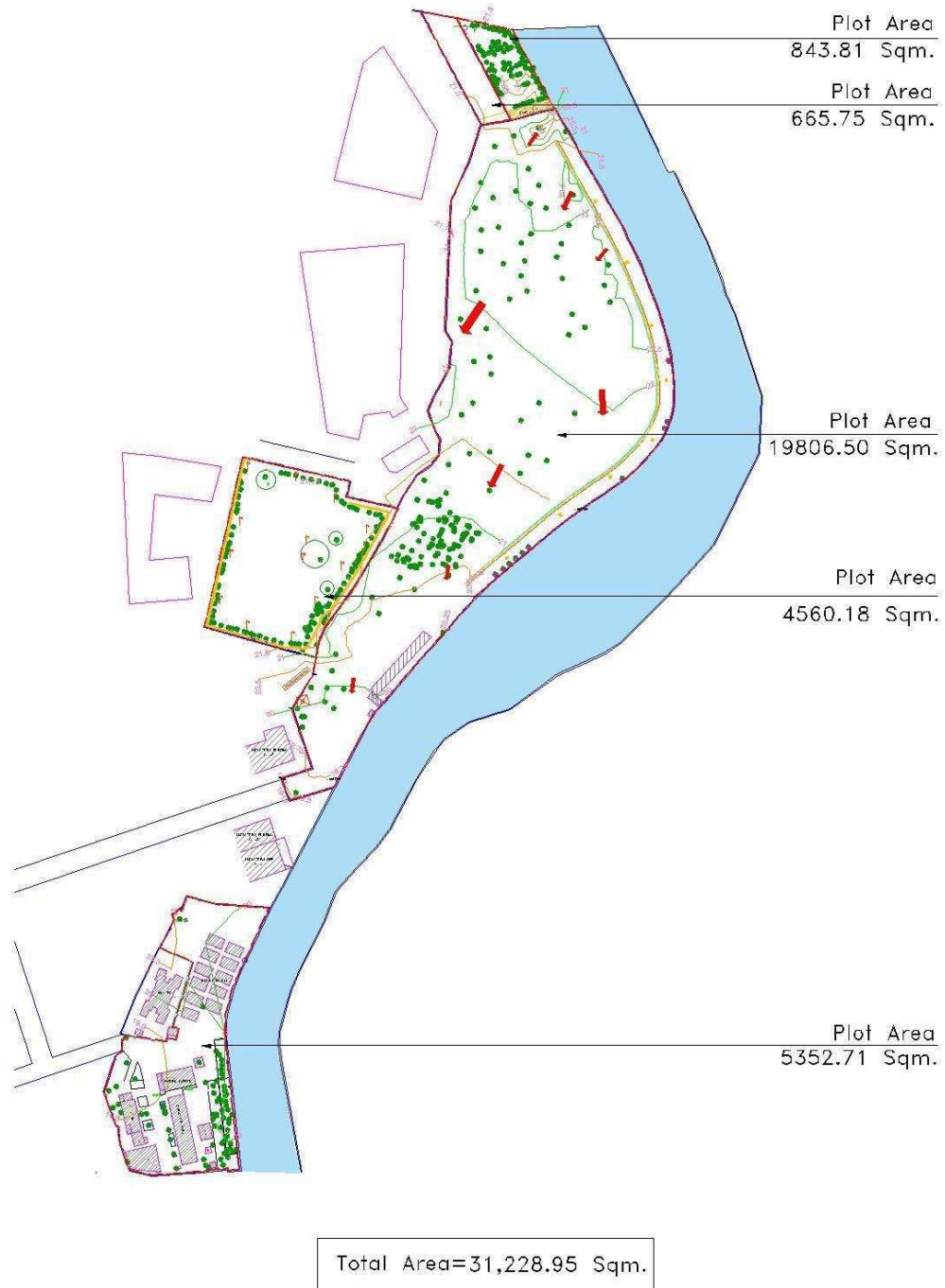
Figure 4: Total Station Survey drawing
